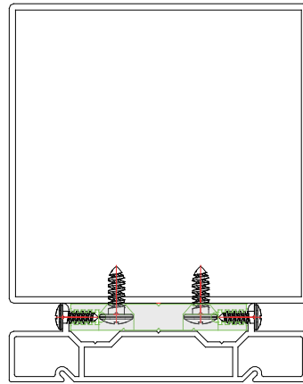
Section
