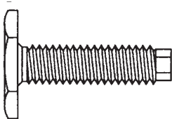
3/4" Hex x 5/16-18 x 1 1/4" Max Hex Stem/Base Glide
