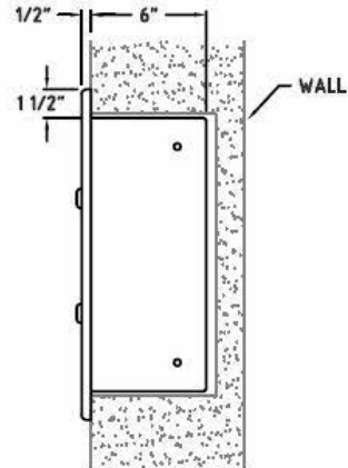
FLUSH MOUNT HGF
