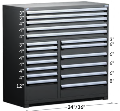
18 DRAWERS R5KKE-5813 60" × 24" × 60" R5KKG-5813 60" × 27" × 60"
