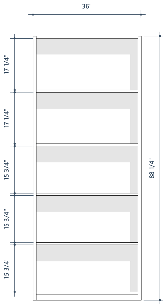
2 Option 4 Front 3/4" = 1'-0"
