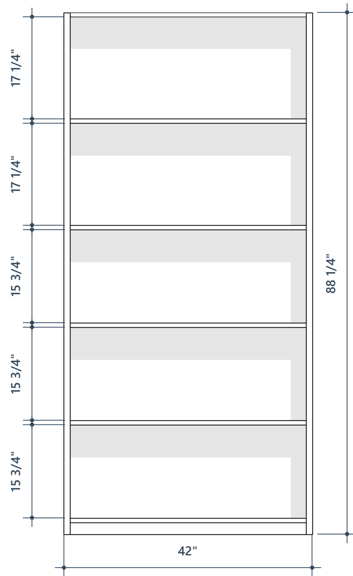
2 Option 3 Front 3/4" = 1'-0"
