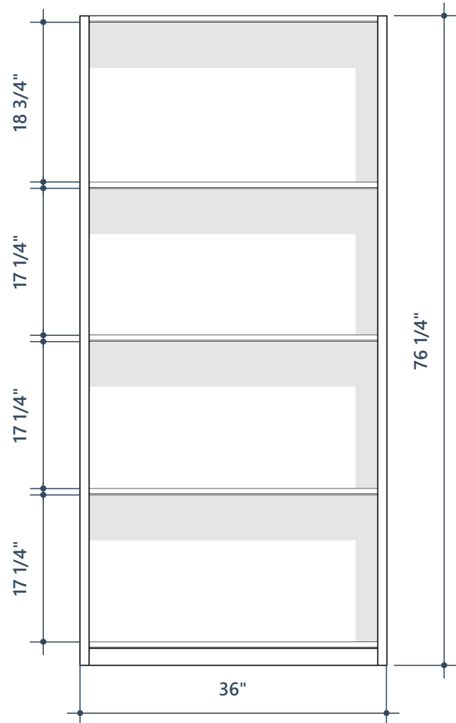
2 Option 1 Front 3/4" = 1'-0"
